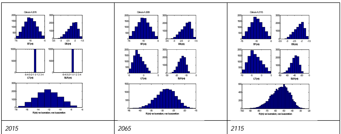
Figure 31-8 Histograms of parameter samples and the resultant shoreline distances for 2015, 2065 and 2115 timeframes for cell 31G
