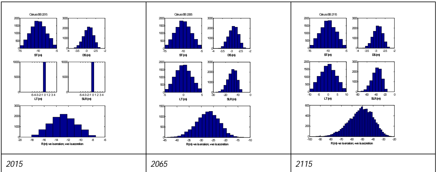
Figure 31-3 Histograms of parameter samples and the resultant shoreline distances for 2015, 2065 and 2115 timeframes for cell 31BB
