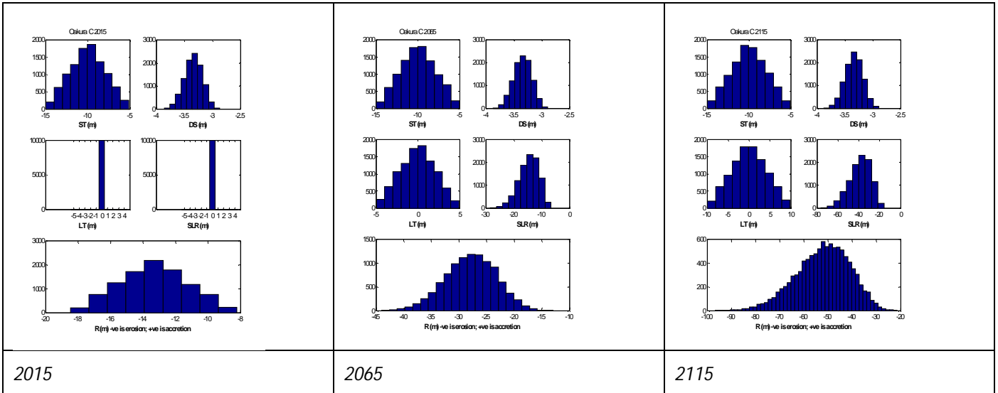
Figure 31-4 Histograms of parameter samples and the resultant shoreline distances for 2015, 2065 and 2115 timeframes for cell 31C
