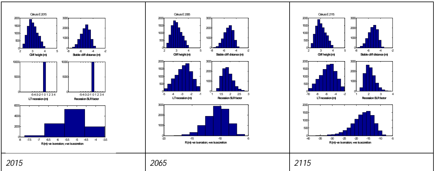
Figure 31-6 Histograms of parameter samples and the resultant shoreline distances for 2015, 2065 and 2115 timeframes for cell 31E
