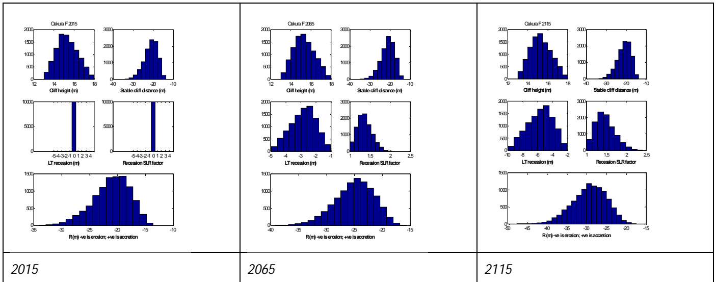
Figure 31-7 Histograms of parameter samples and the resultant shoreline distances for 2015, 2065 and 2115 timeframes for cell 31F
