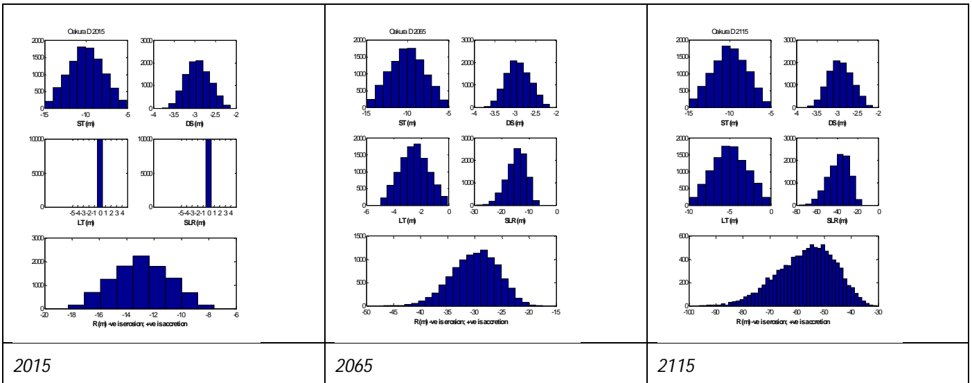
Figure 31-5 Histograms of parameter samples and the resultant shoreline distances for 2015, 2065 and 2115 timeframes for cell 31D
