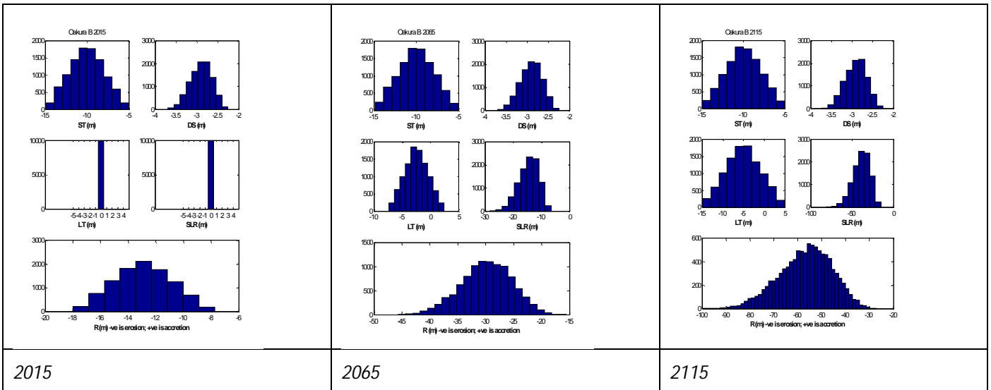
Figure 31-2 Histograms of parameter samples and the resultant shoreline distances for 2015, 2065 and 2115 timeframes for cell 31B
