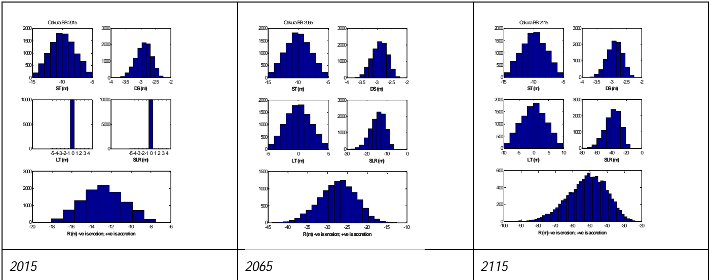
Figure 31-10 Histograms of parameter samples and the resultant shoreline distances for 2015, 2065 and 2115 timeframes for cell 31I
