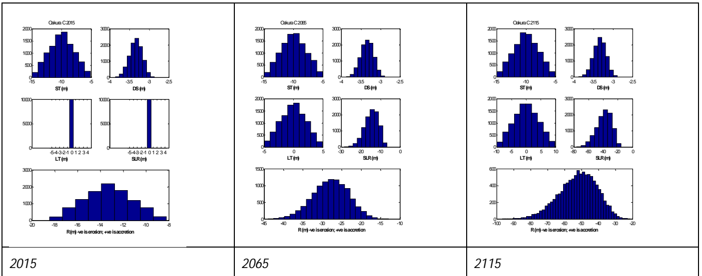
Figure 31-11 Histograms of parameter samples and the resultant shoreline distances for 2015, 2065 and 2115 timeframes for cell 31J
