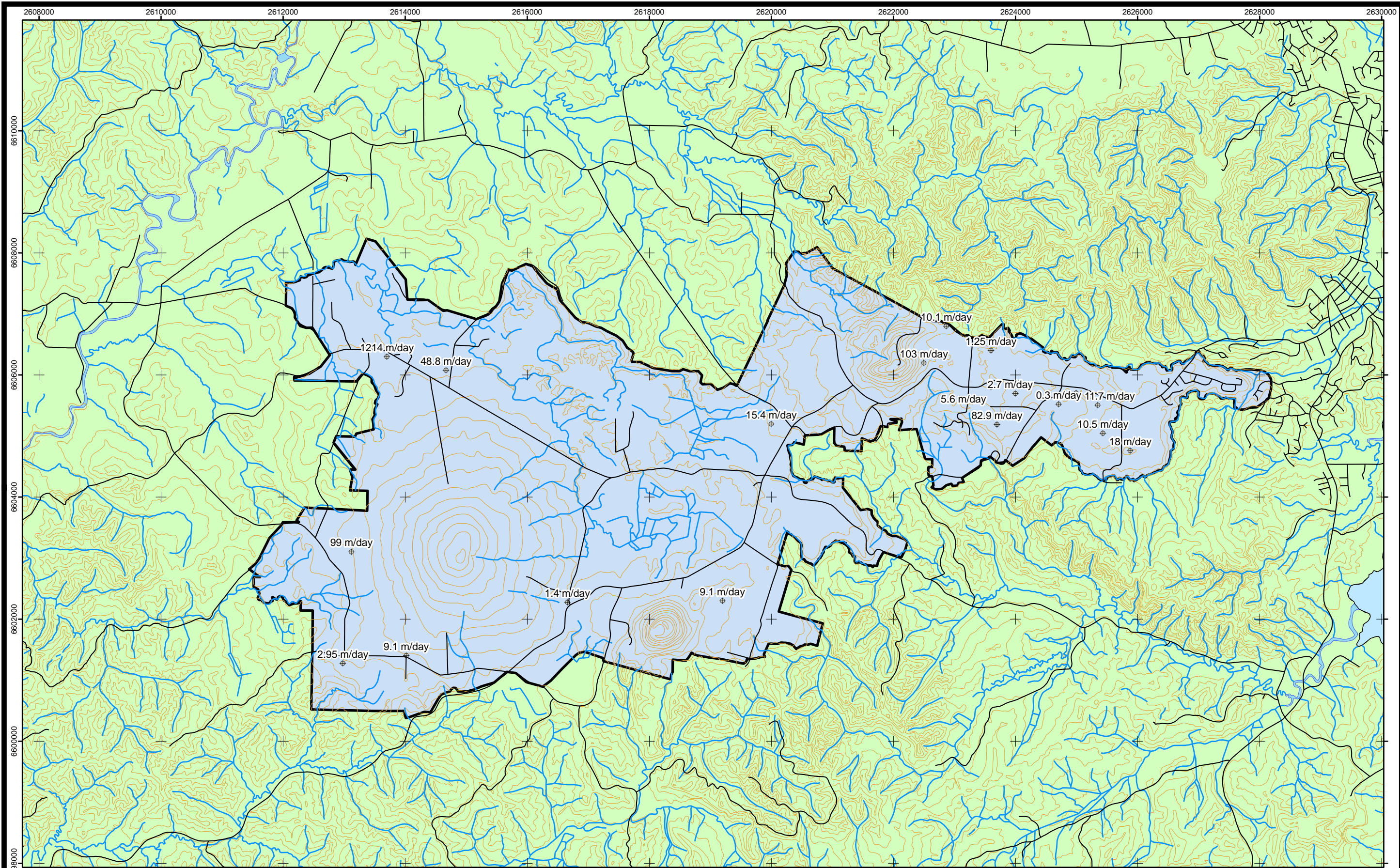
Hydraulic Conductivity Values Within the Study Area Figure 14
