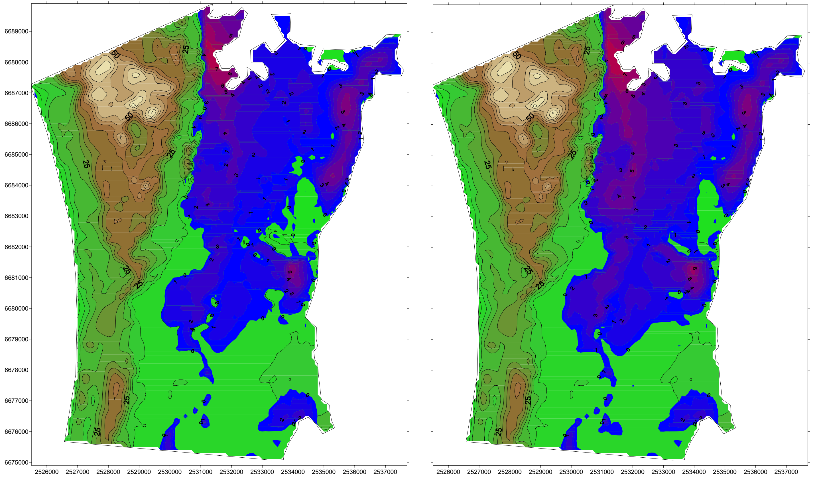
Figure 37. Extent of artesian pressures in model Layer 4 for a) status quo and b) capping of artesian bores.
