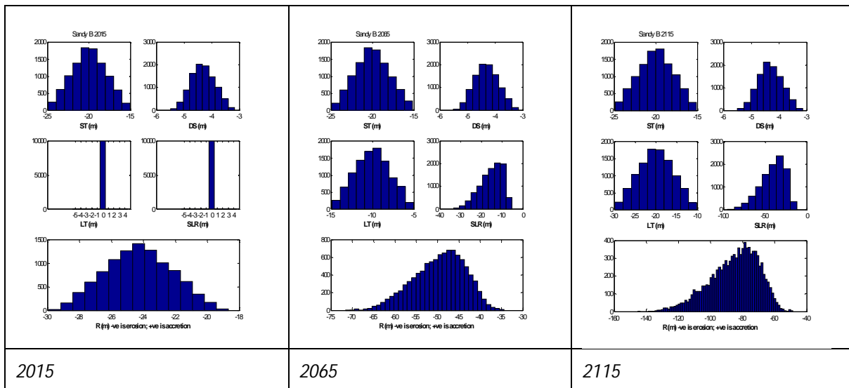
Figure 12-3 Histograms of parameter samples and the resultant shoreline distances for 2015, 2065 and 2115 timeframes for cell 12B
