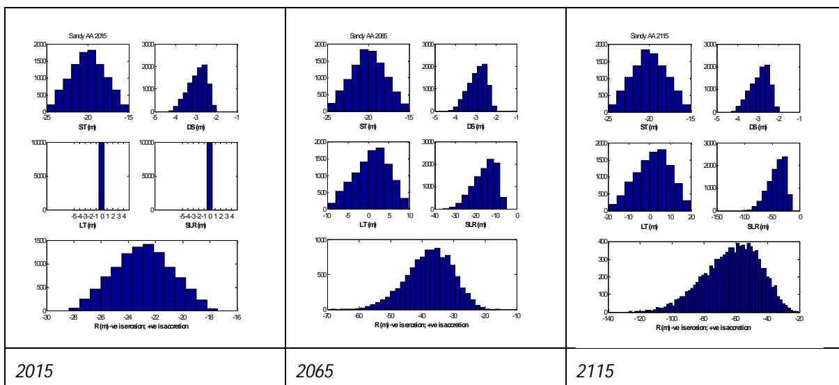
Figure 12-2 Histograms of parameter samples and the resultant shoreline distances for 2015, 2065 and 2115 timeframes for cell 12AA
