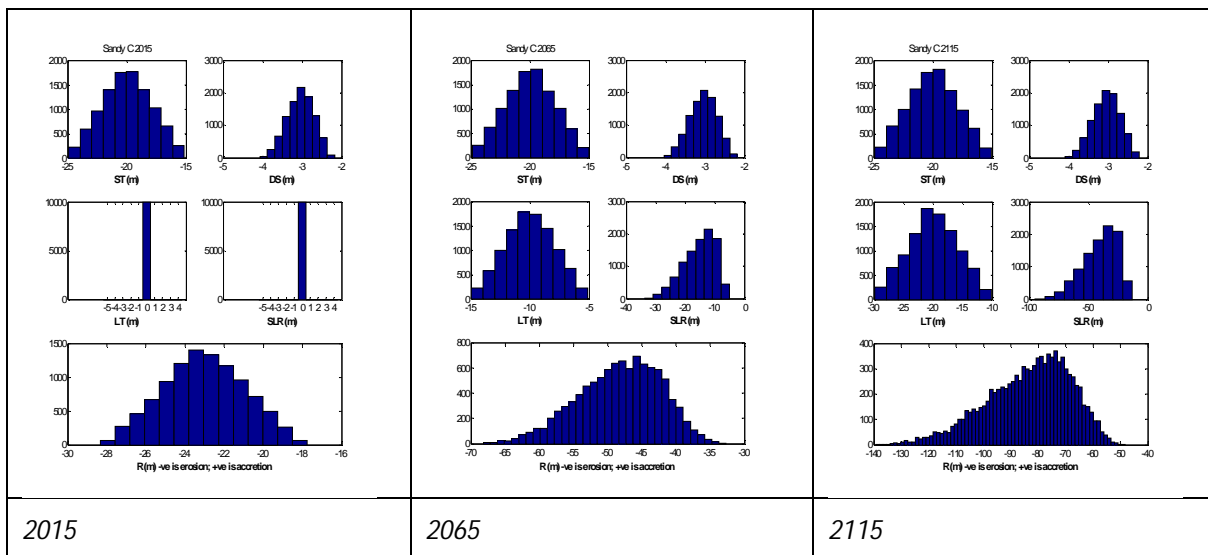
Figure 12-4 Histograms of parameter samples and the resultant shoreline distances for 2015, 2065 and 2115 timeframes for cell 12C
