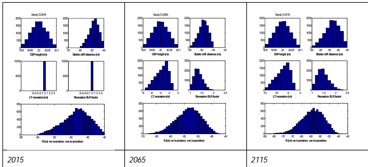
Figure 12-5 Histograms of parameter samples and the resultant shoreline distances for 2015, 2065 and 2115 timeframes for cell 12D
