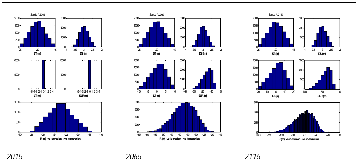
Figure 12-1 Histograms of parameter samples and the resultant shoreline distances for 2015, 2065 and 2115 timeframes for cell 12A
