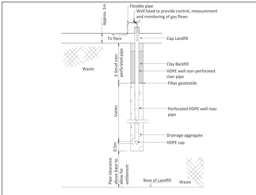
Figure B-4 Typical Landfill Gas Well Design
