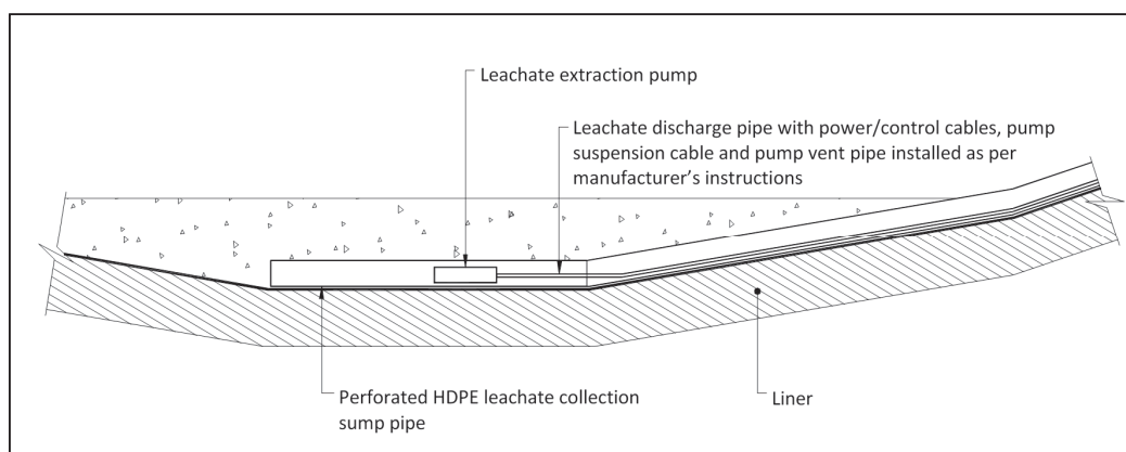
Figure B-2 Inclined Leachate Collection Sump and Riser Going up the Side Slope
