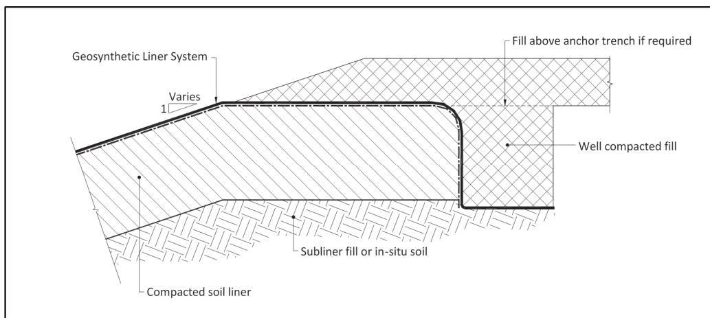
Figure B-1 Typical Anchor Trench Detail
