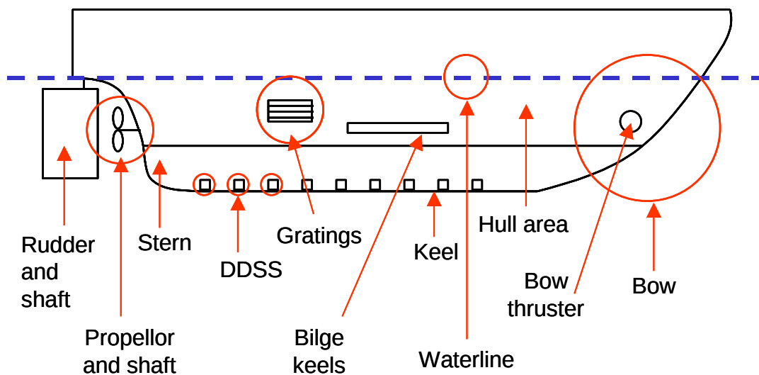
Fig. 2: Target areas on a vessel hull to estimate LoF by diving.
