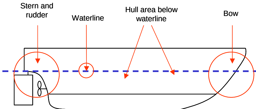
Fig. 1: Target areas on a vessel hull to estimate LoF ranks by surface observation (above-water).
