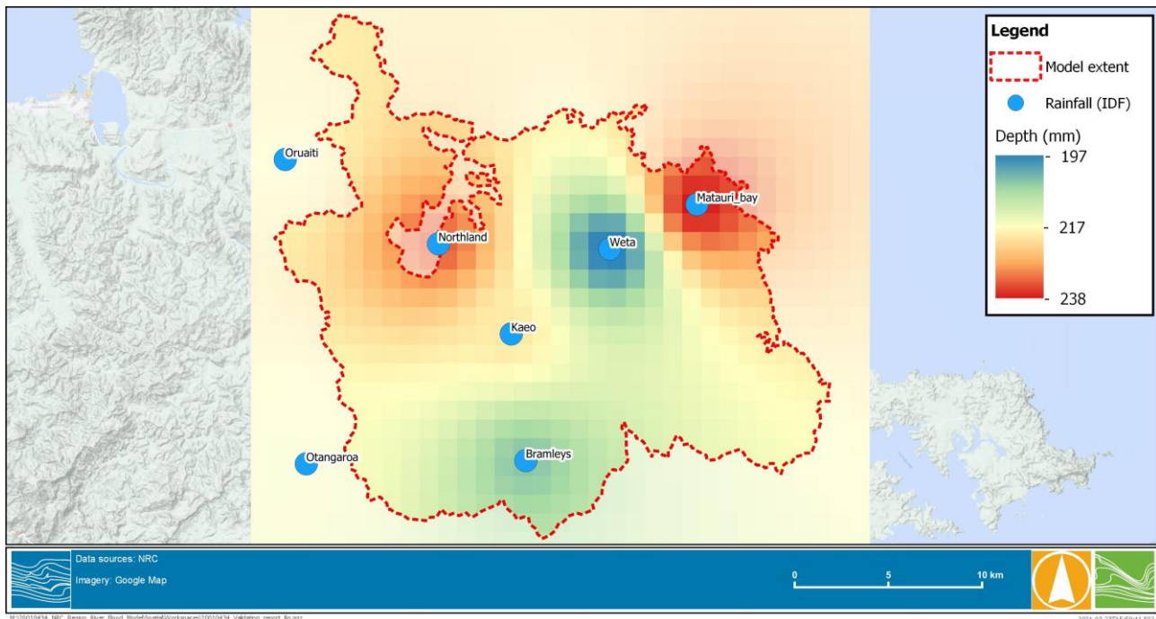
FIGURE 4-1 EXAMPLE OF DESIGN RAINFALL GRID (12-HOUR, 1% AEP RAINFALL) FOR M06
