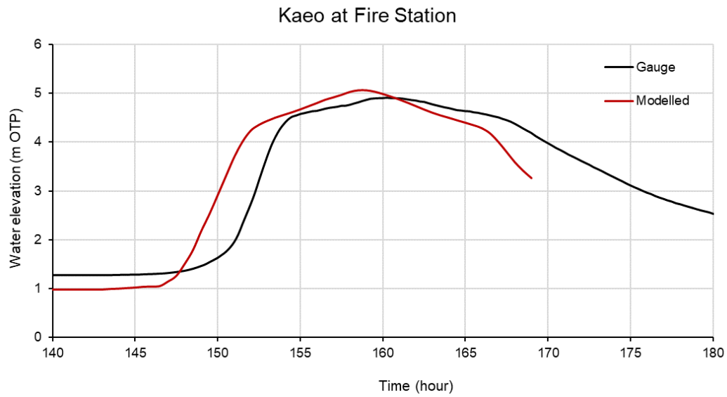
FIGURE 3-3 MODELLED AND GAUGED LEVELS AT KAEO AT FIRE STATION GAUGE
