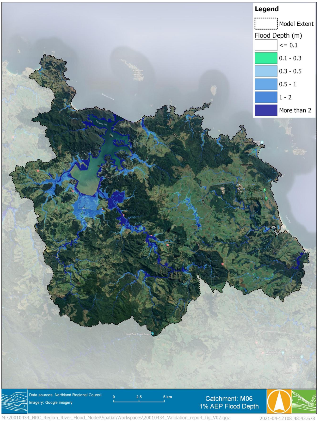
FIGURE 5-1 DESIGN MODELLING OF 1% AEP FLOOD DEPTH
