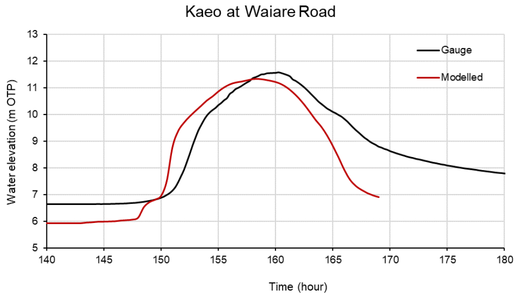
FIGURE 3-1 MODELLED AND GAUGED LEVELS AT KAEO AT WAIARE ROAD GAUGE
