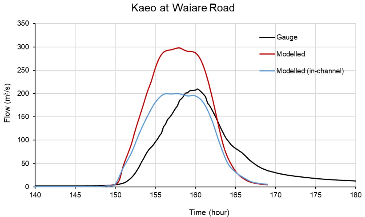
FIGURE 3-2 MODELLED AND GAUGED FLOWS AT KAEO AT WAIARE ROAD GAUGE
