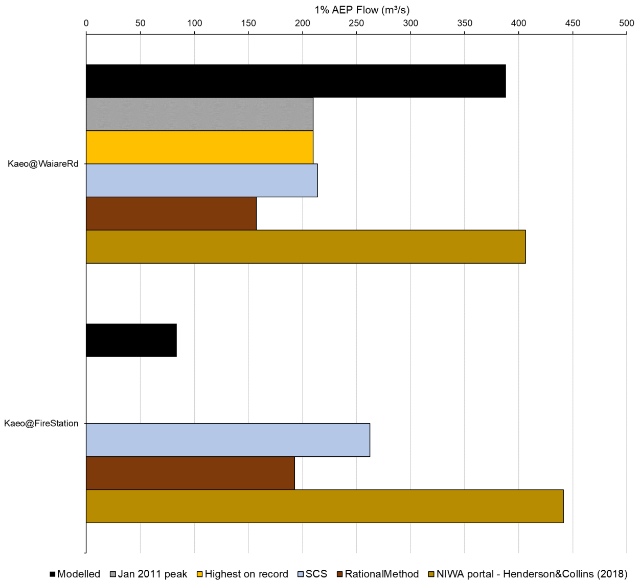
FIGURE 6-2 VERIFICATION OF DESING MODELLING RESULTS AGAINST HYDROLOGICAL ESTIMATES
