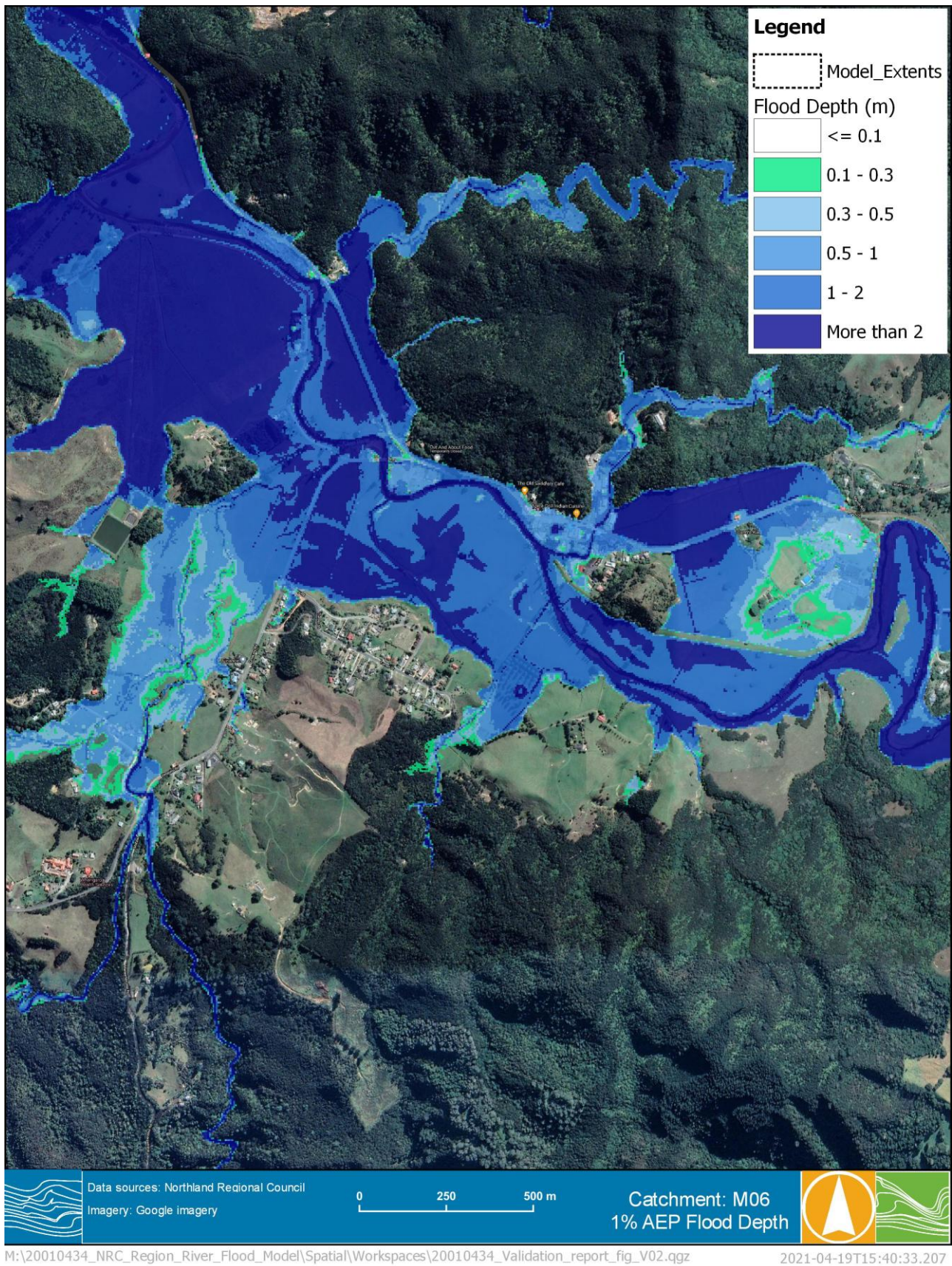
FIGURE 5-4 DESIGN MODELLING OF 1% AEP FLOOD DEPTH AT KAE0
