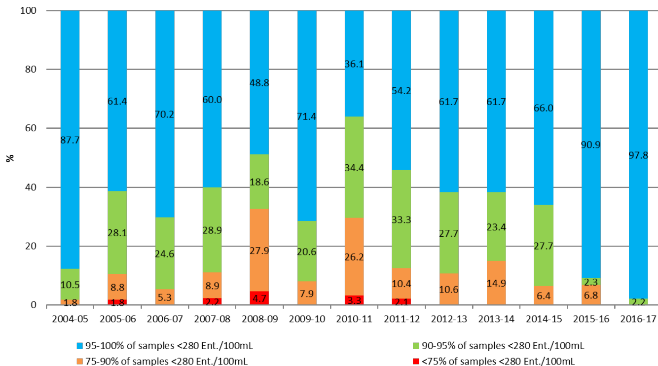
Figure 2: Yearly overall percentage of coastal sites with corresponding percentage of samples within each category from 2004 to 2017
