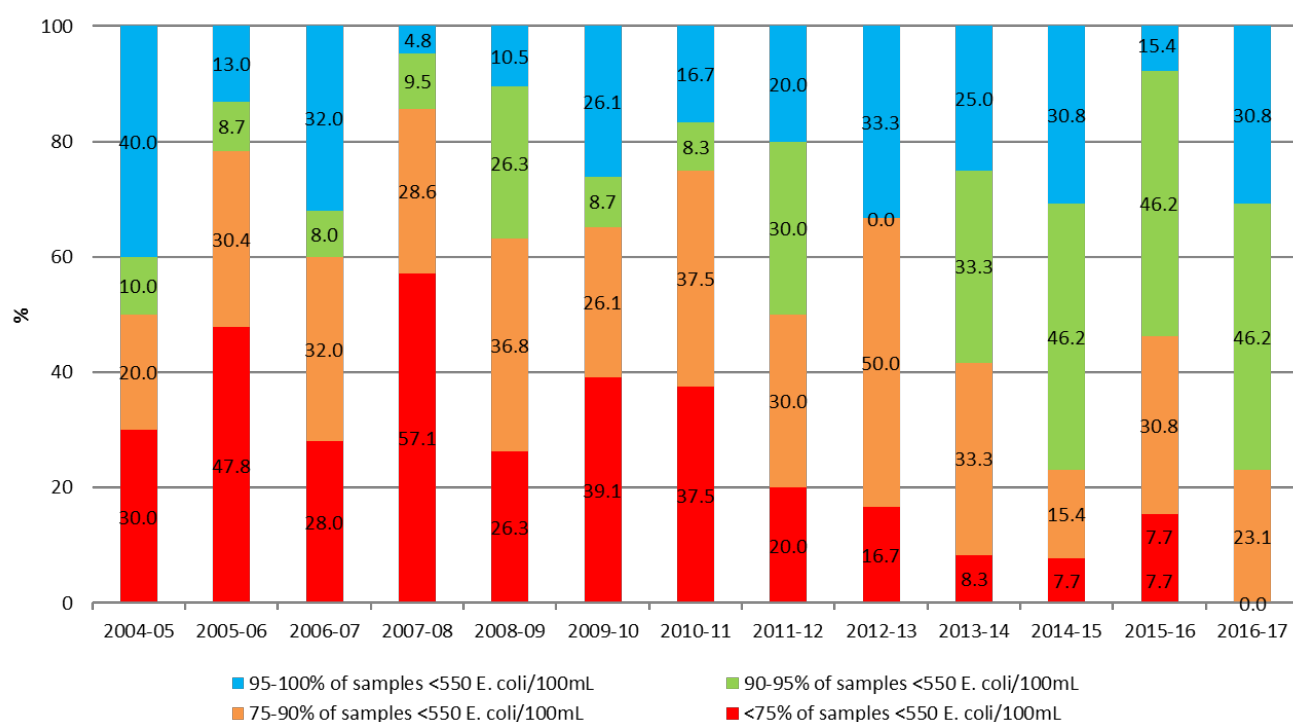
Figure 4: Yearly overall percentage of freshwater sites with corresponding percentage of samples within each category from 2004 to 2017
