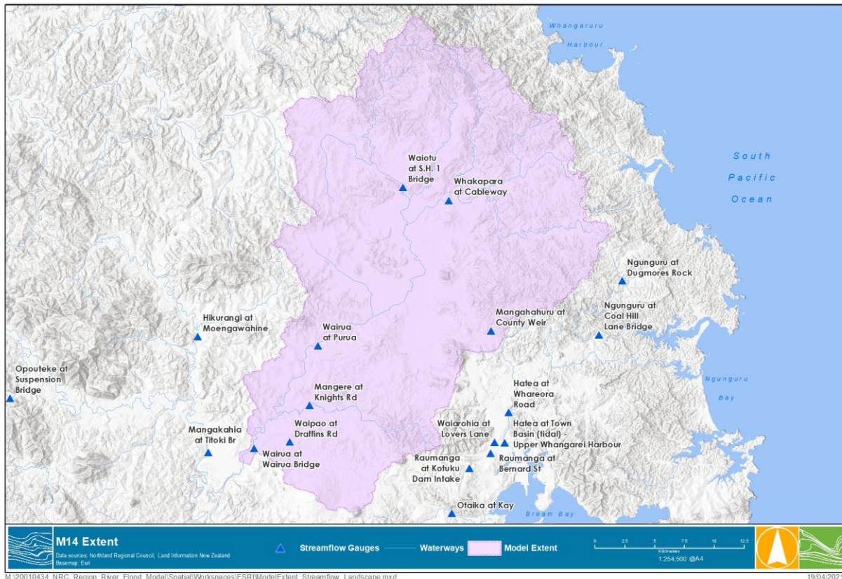
FIGURE 5-1 AVAILABLE STREAMFLOW GAUGES WITHIN LOWER PURUA, LOWER WAIUABRIDGE, MANGAHAHURU, MANGERE, WAIPAO, WAIOTU, WHAKAPARA CATCHMENT
