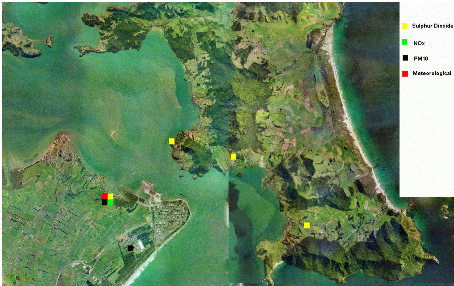
■ Figure 4.1 – Recommended Ambient Air and Meteorological Monitoring Sites
