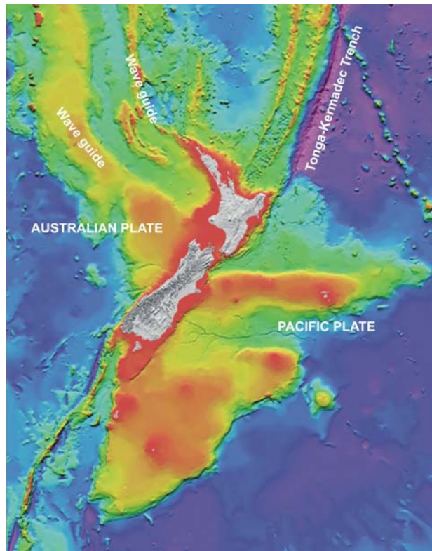
Figure 1: Geophysical setting of New Zealand showing the Tonga-Kermadec Trench (taken from Goff et al. 2006).
