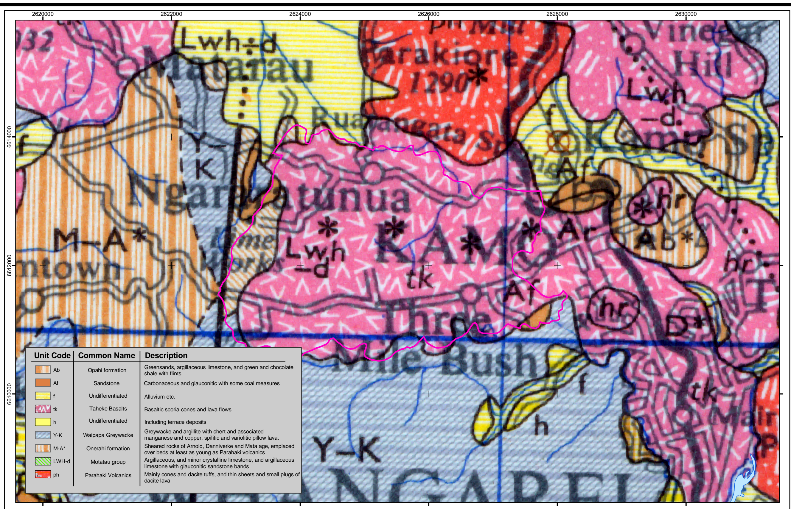
Regional Geology Three Mile Bush FIGURE 3.
