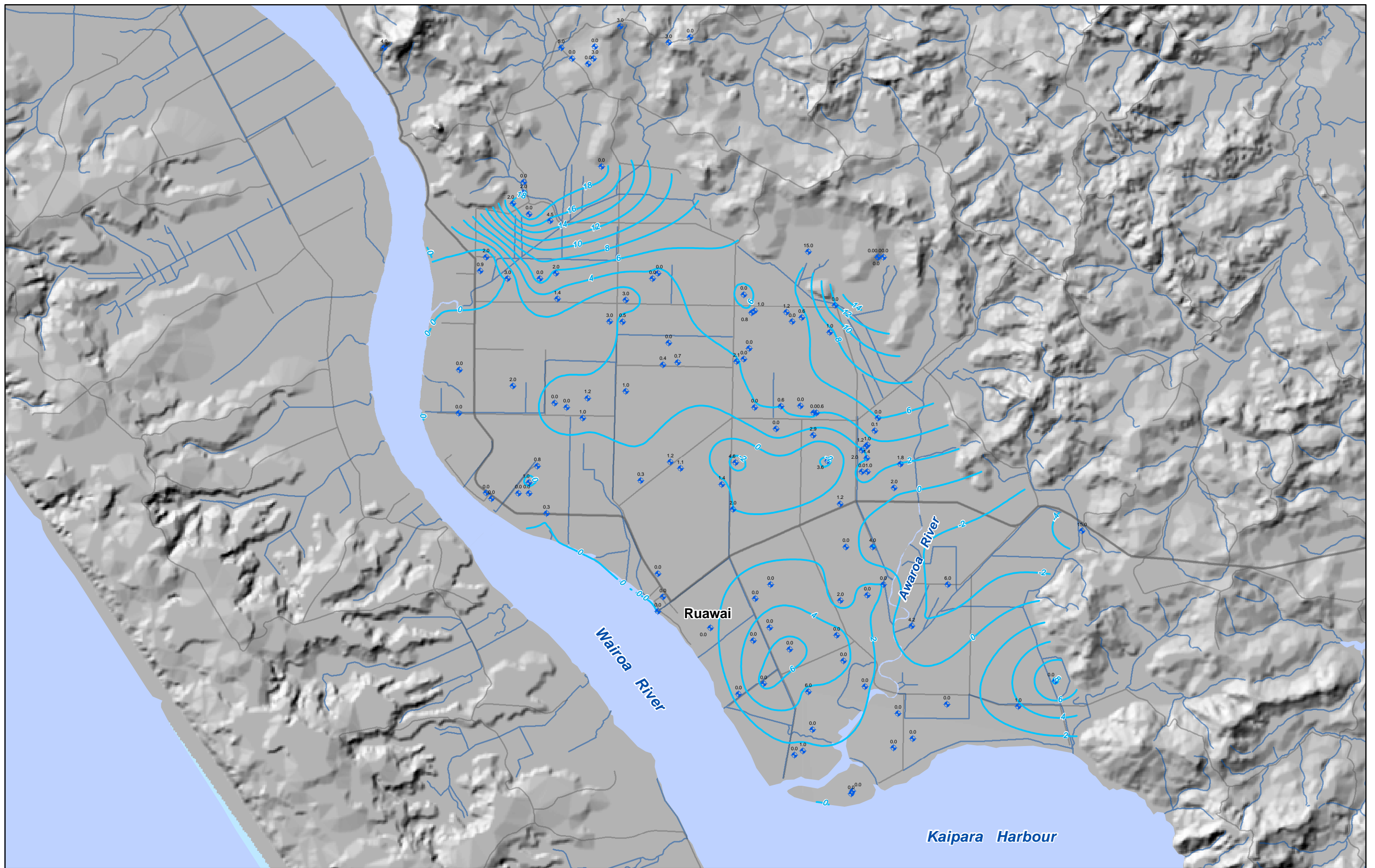
Figure 9. Piezometric Surface Ruawai Plains
