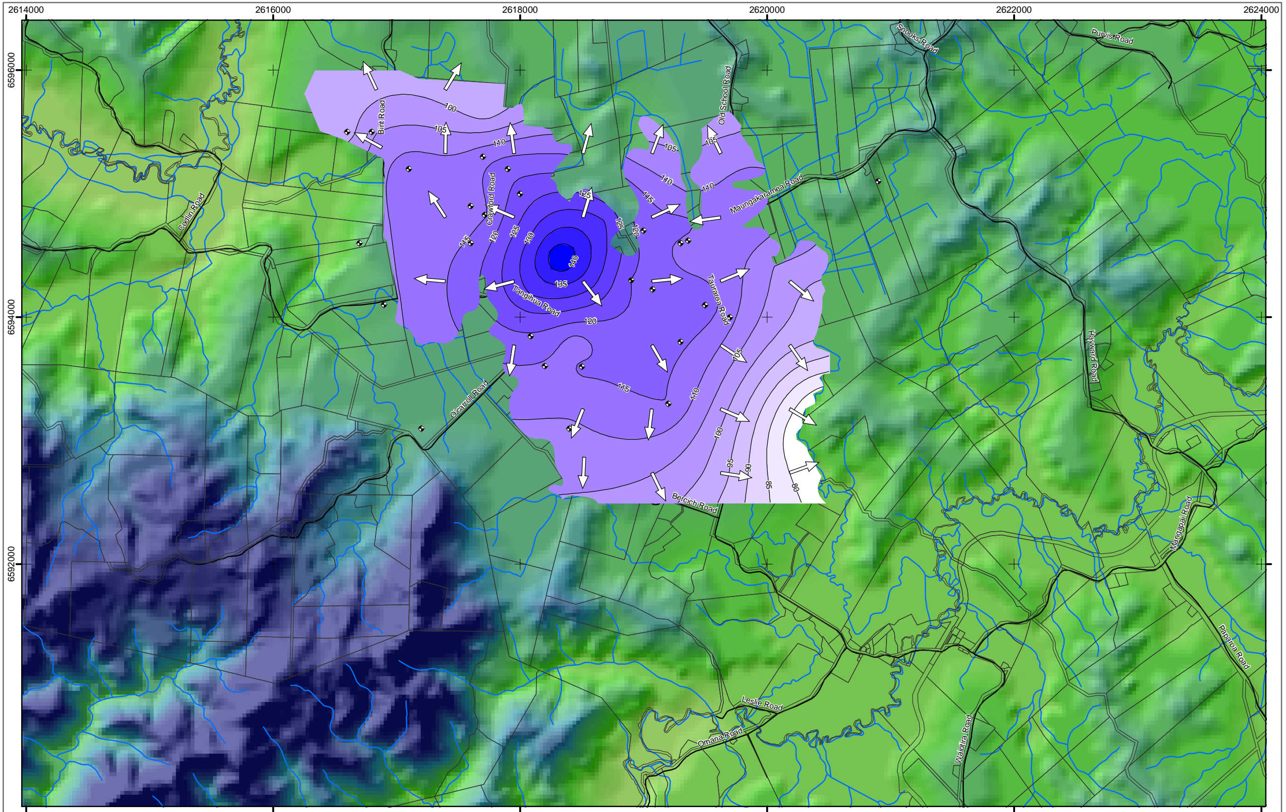
Maungakarema Piezometric Surface FIGURE 7.
