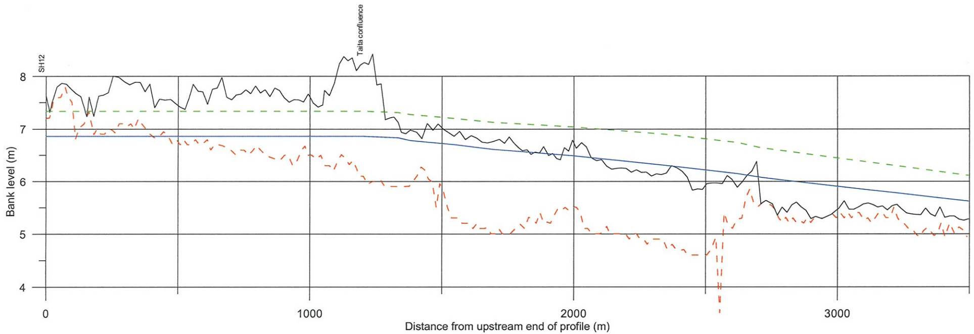
Taita Stream right bank and Kaihu right bank Maitahi to Bottleneck (survey RB4) - - - Estimated natural unmodified bank level — Bank crest surveyed 2010 — Maximum water level in 6 month ARI flood, with no bank overtopping - - - Maximum water level in 1 year ARI flood, with no bank overtopping
