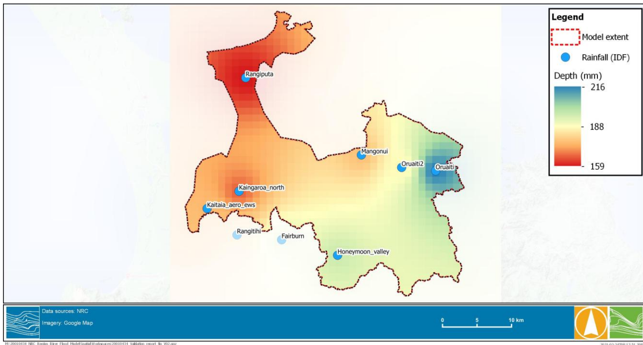
FIGURE 3-1 EXAMPLE OF DESIGN RAINFALL GRID (12-HOUR, 1% AEP RAINFALL) FOR M09
