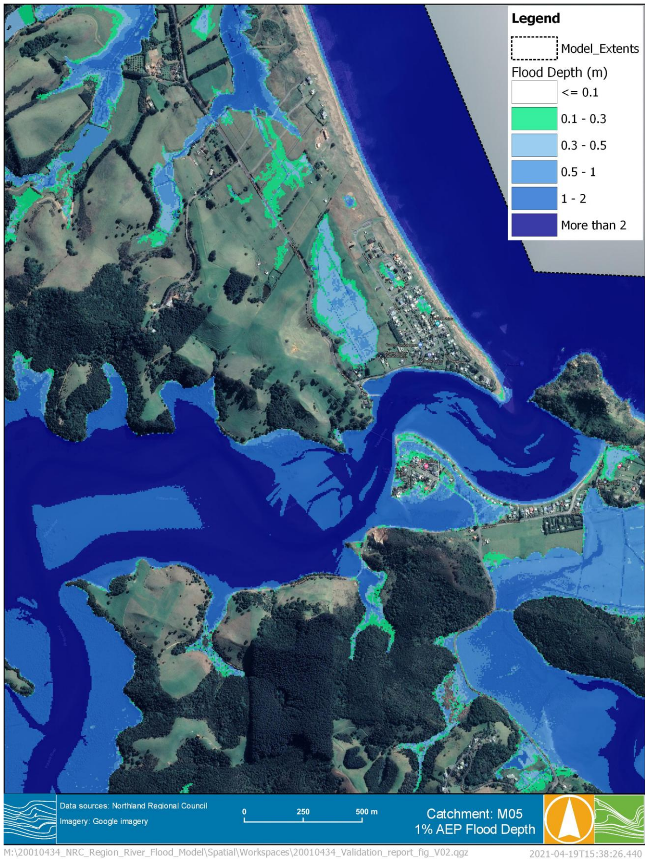
FIGURE 4-4 DESIGN MODELLING OF 1% AEP FLOOD DEPTH ZOOMED AT PATAUA
