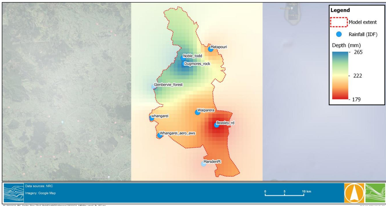
FIGURE 3-1 EXAMPLE OF DESIGN RAINFALL GRID (12-HOUR, 1% AEP RAINFALL) FOR M05
