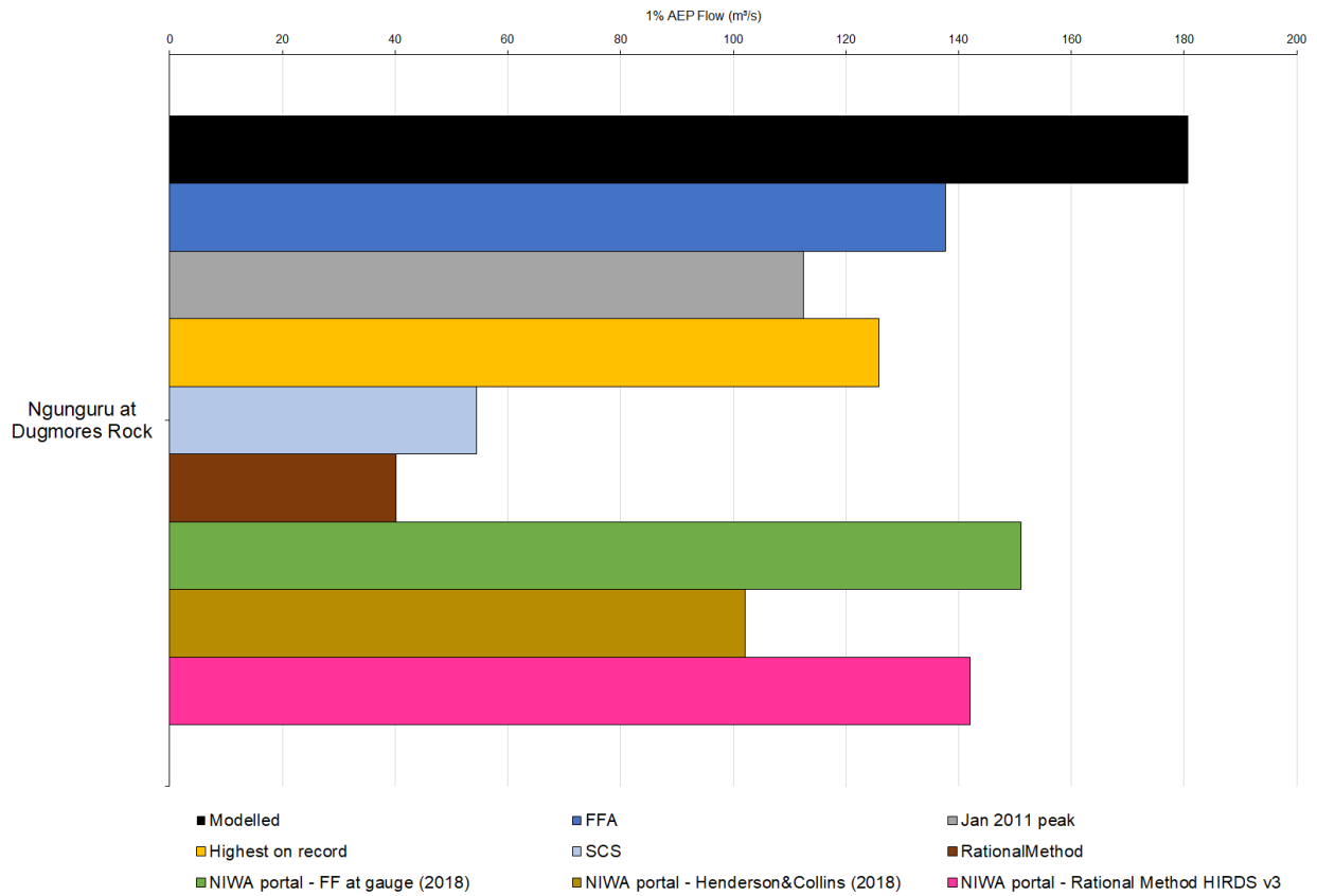
FIGURE 5-3 VERIFICATION OF DESIGN MODELLING RESULTS AGAINST HYDROLOGICAL ESTIMATES
