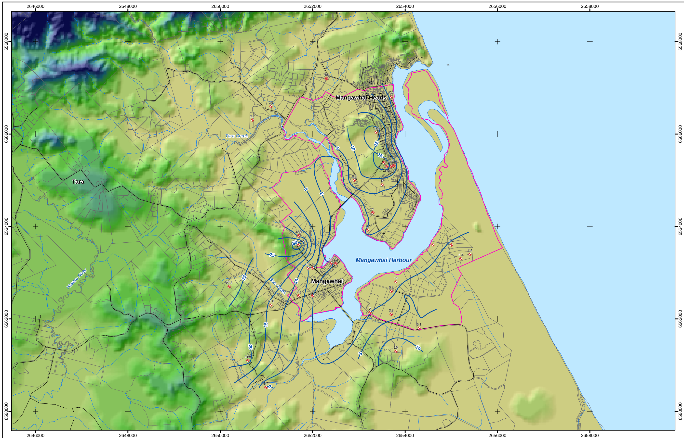
Piezometric Surface Waitemata Aquifer FIGURE 9.
