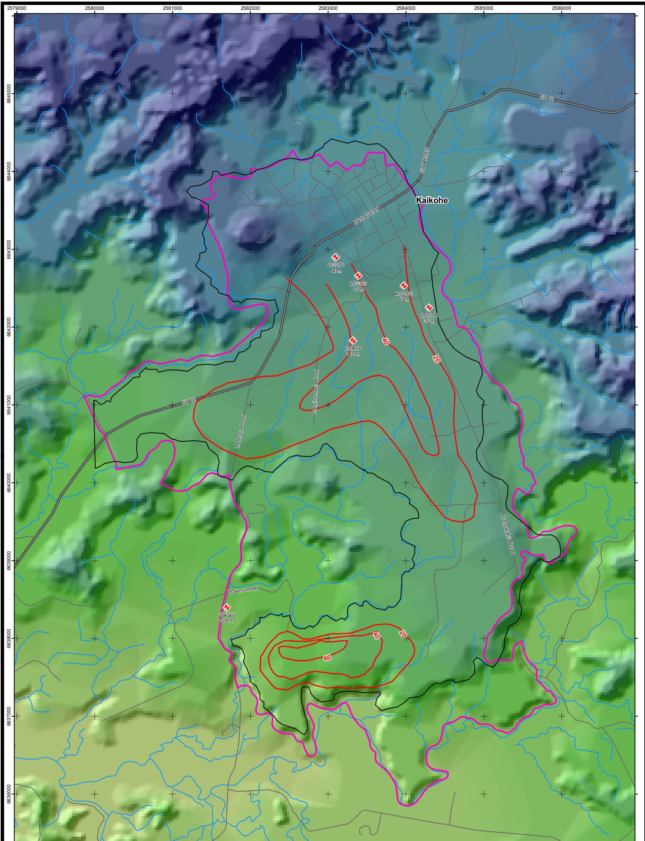
Basalt Thickness Map Figure 5.
