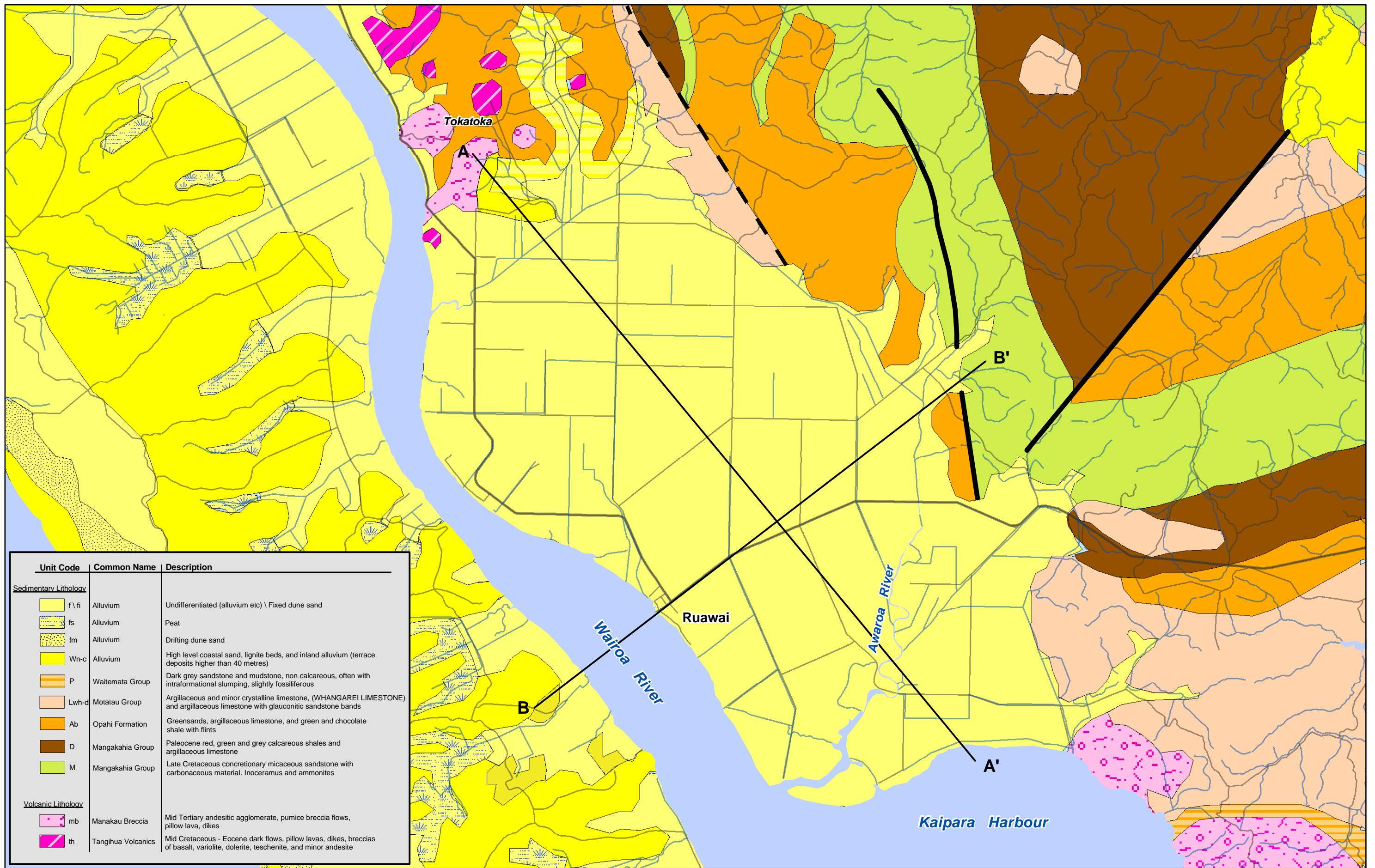
Figure 2. Regional Geology Ruawai Plains
