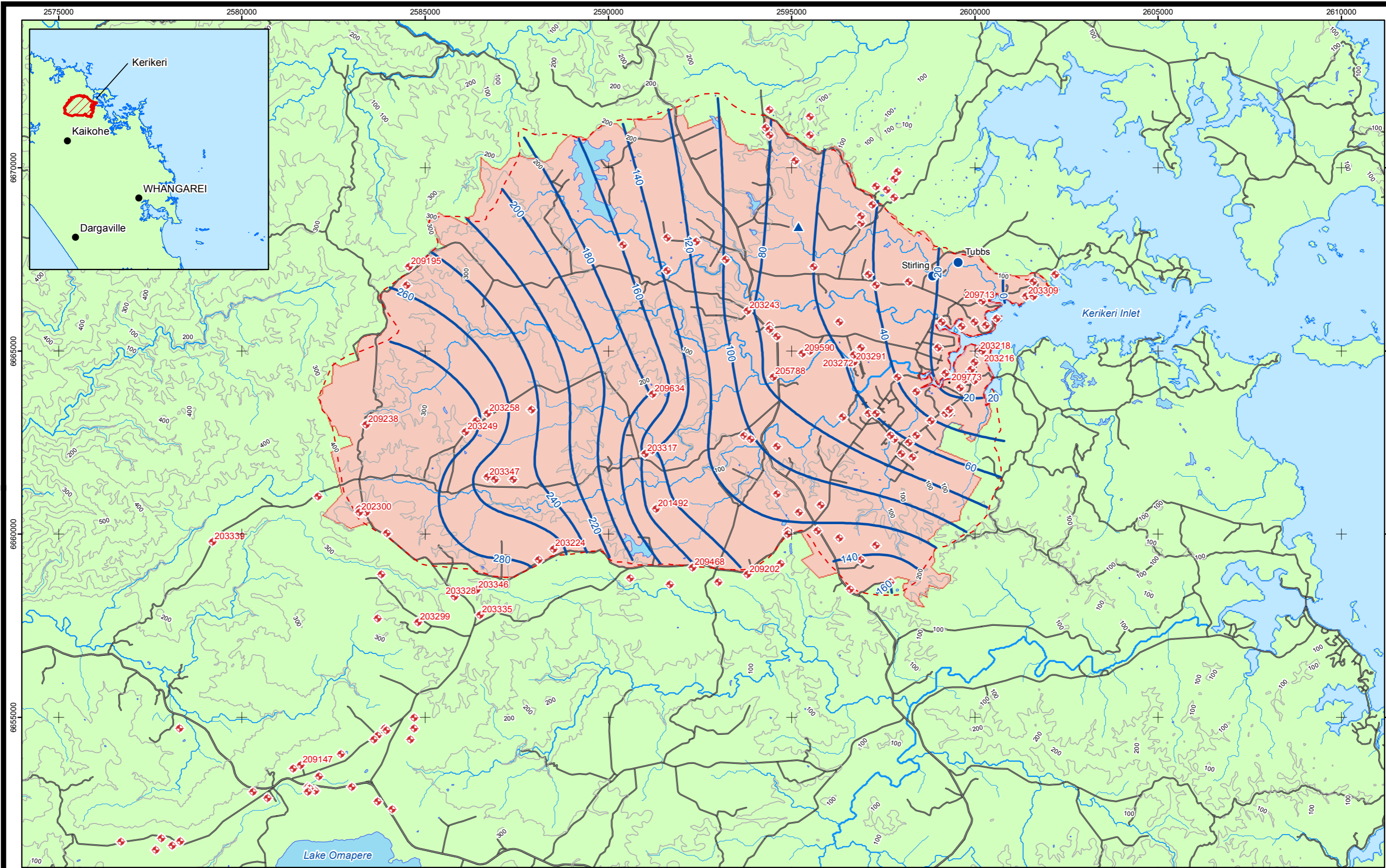
Kerikeri Basalt Piezometric Surface Map Figure 4.
