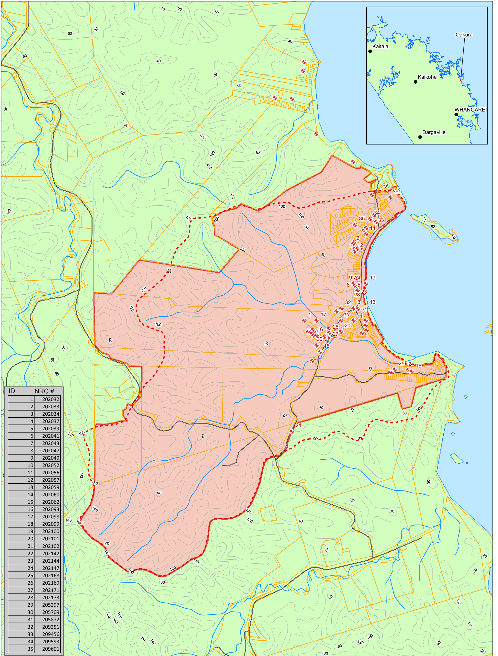
Oakura Greywacke Aquifer Management Map Figure 2
